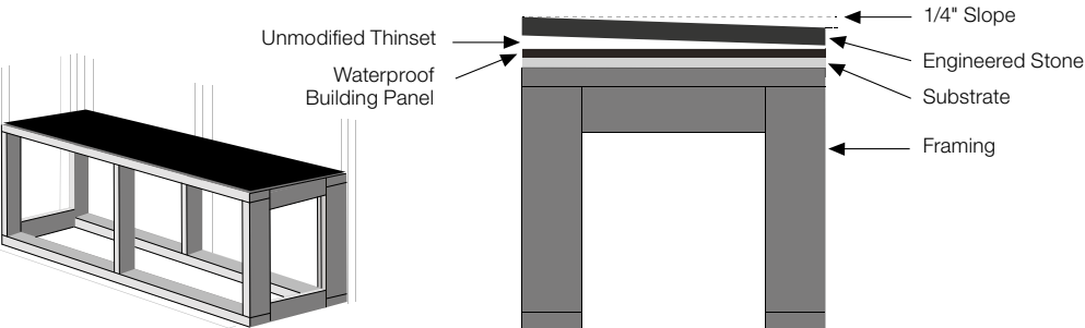
Installation Diagram
