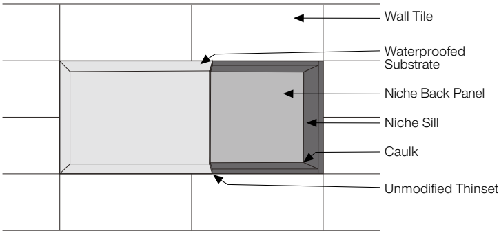
Fig.1 Installation Diagram
