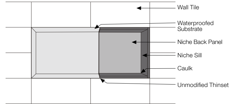
Installation Diagram
