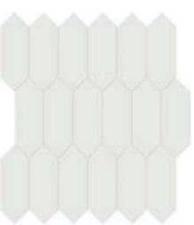
2 x 5 in / 4.6 x 12.8 cm Picket Mosaic Actual: 284 x 318 x 6 mm Glossy: BFS25PGVG Matte: BFS25PMVG
